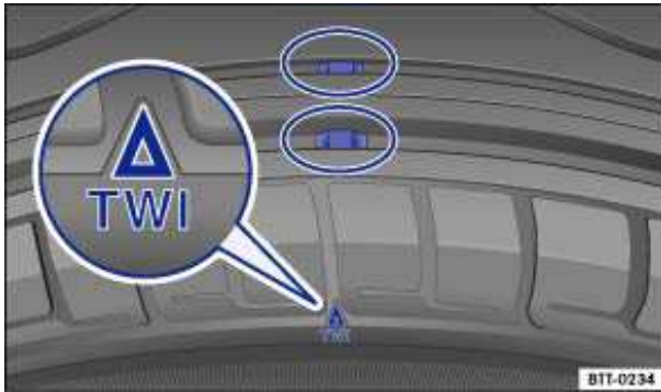
Fig. 124 Tread pattern: Wear indicator.
