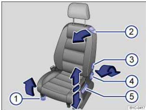
Fig. 33 Controls on the left front seat.
