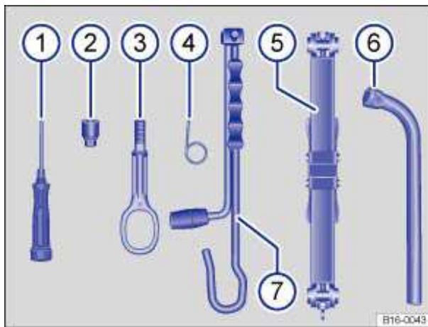
Fig. 136 Contents of the vehicle tool kit.
