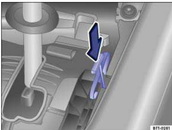
Fig. 134 Releasing the selector lever lock.
