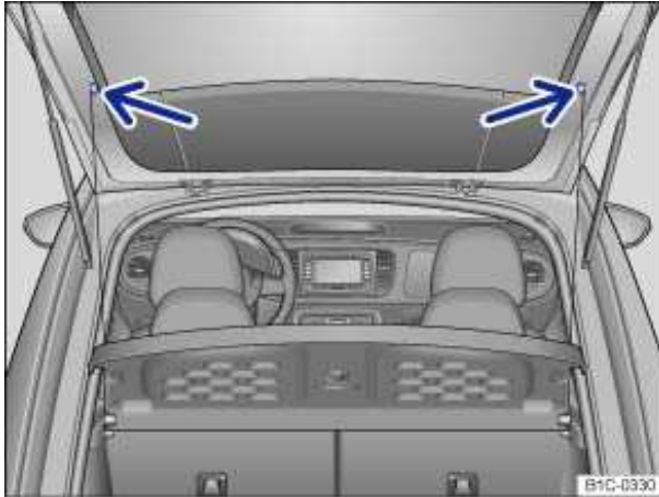
Fig. 77 On the rear hatch: Installing and removing the supporting cords.
