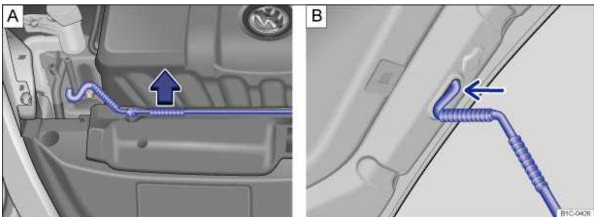
Fig. 115 A: Bracket for hood support in the engine compartment. B: Hood propped open.
