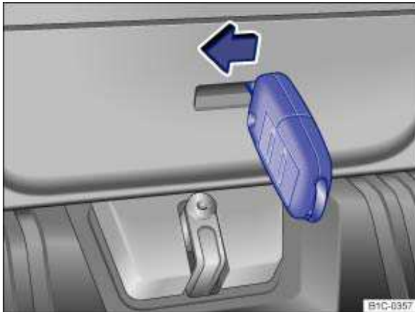
Fig. 132 View from luggage compartment: Opening the rear hatch.
