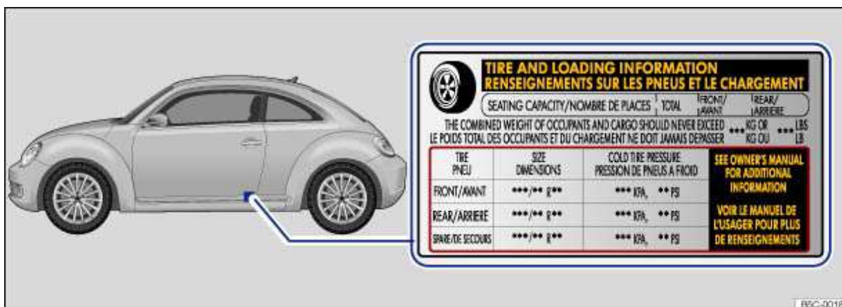
Fig. 123 Location of the tire inflation pressure label.
