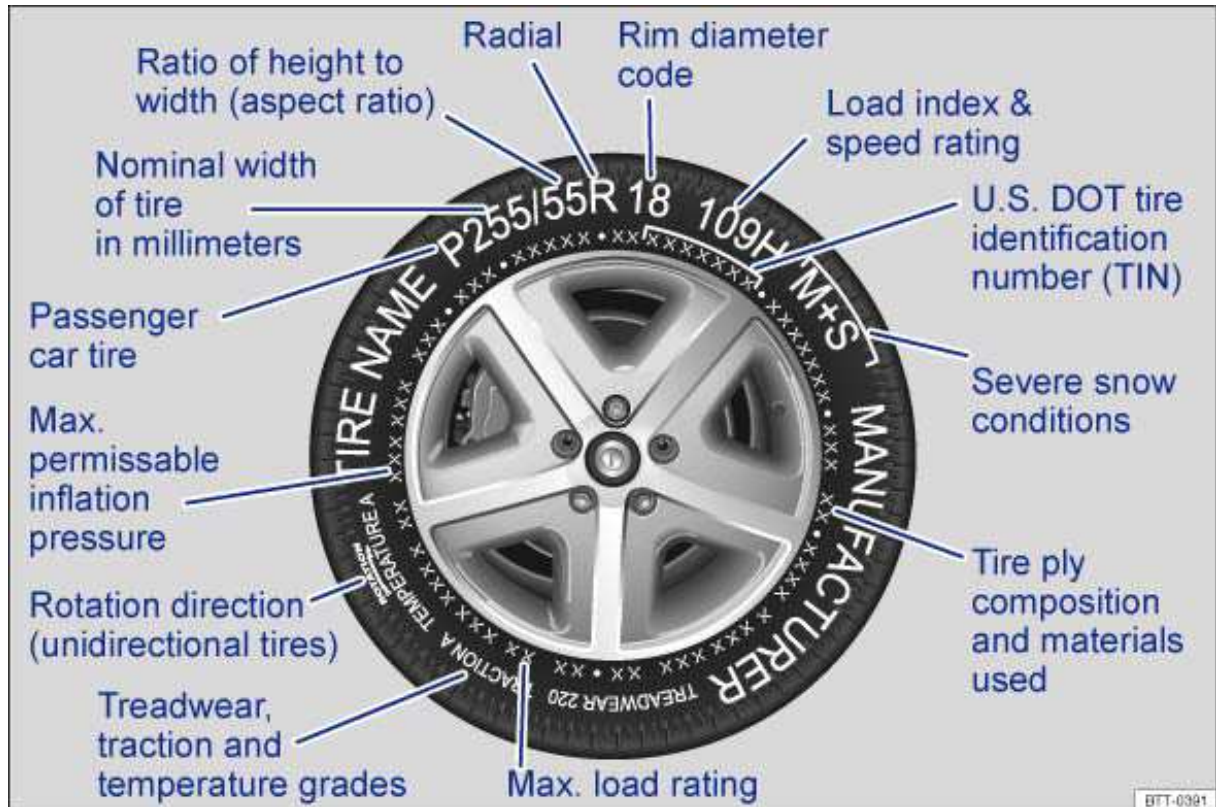
Fig. 126 International tire labeling.
