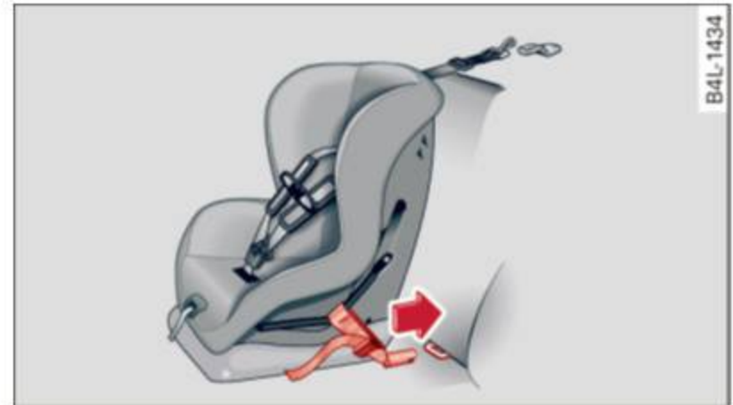
Fig. 122 Lower anchorages: proper mounting
