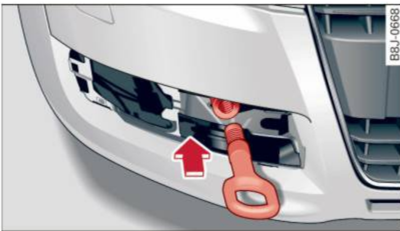
Fig. 171 Front bumper: screwing in the towing loop
