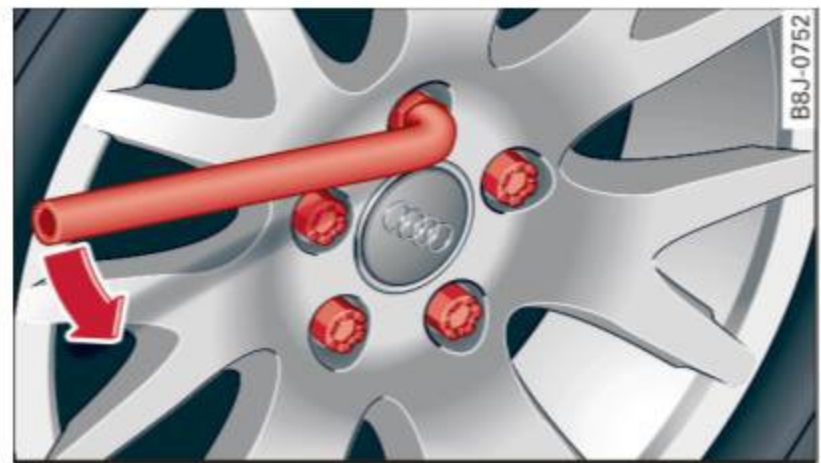
Fig. 159 Wheel change: loosening the wheel bolts
