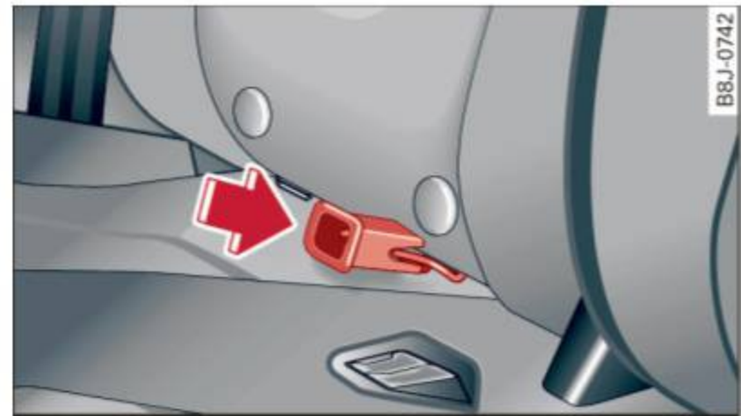
Fig. 121 Close-up: fitting the guidance fixture over the lower anchorage bracket
