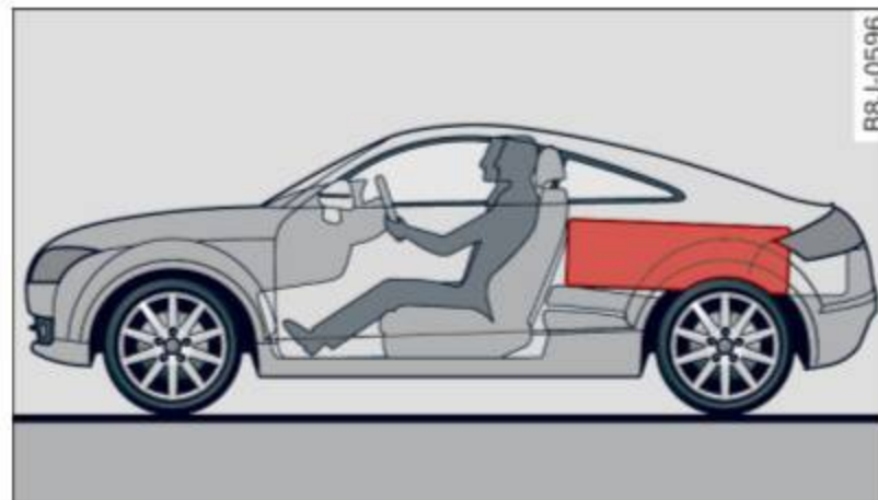
Fig. 93 Safe load positioning: heavy cargo positioned as far forward as possible.
