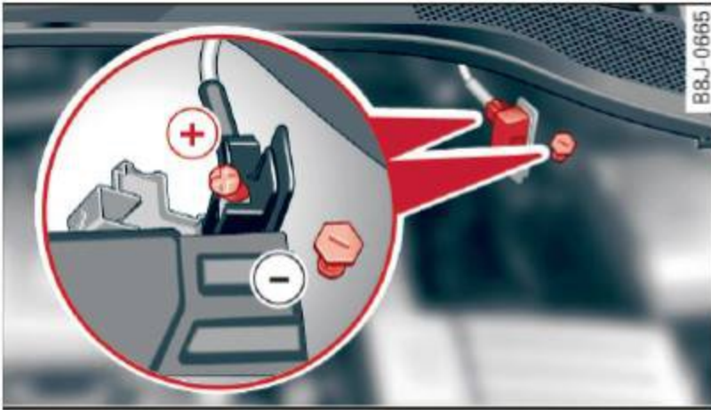
Fig. 168 Engine compartment: Connectors for jumper cables and charger
