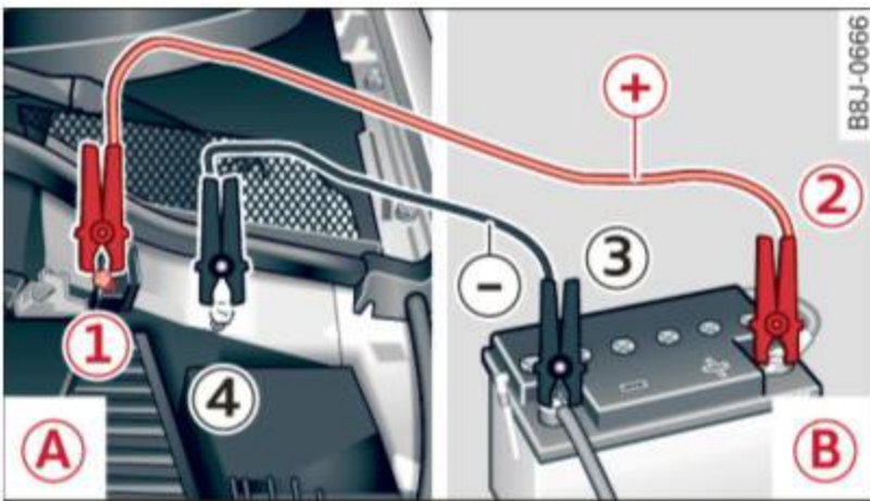
Fig. 169 Jump starting with the battery of another vehicle: (A) discharged vehicle battery, (B) booster battery
