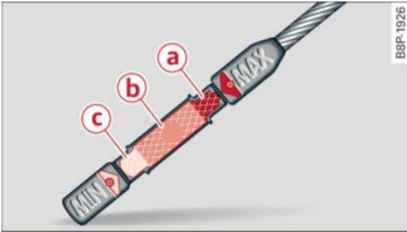
Fig. 135 Illustration of principle 1: Markers on oil dipstick
