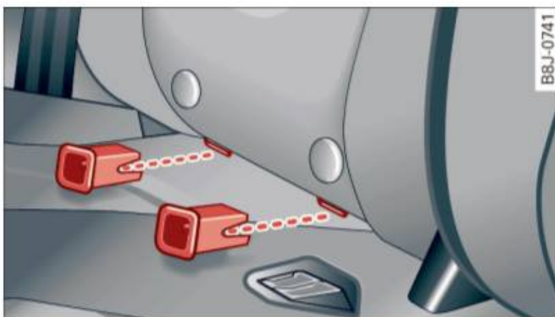
Fig. 120 Rear seats: installing the guidance fixtures
