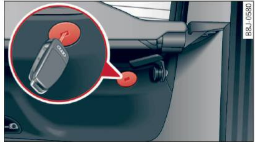
Fig. 34 Access to emergency release on the left side of the luggage compartment below the rear window
