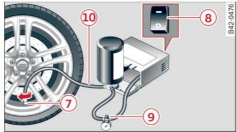
Fig. 156 Connector for the Tire Mobility System
