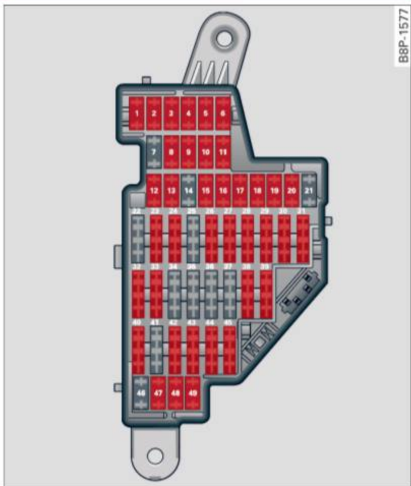
Fig. 166 Fuse carrier behind the instrument panel end face, cover removed
