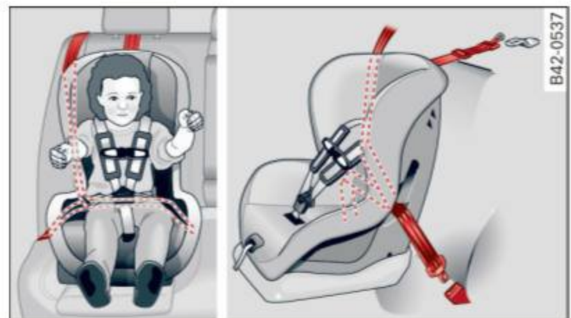
Fig. 115 Schematic overview: installation of the seat using the vehicle's safety belt system
