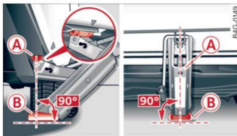
Fig. 161 Sill: positioning the vehicle jack
