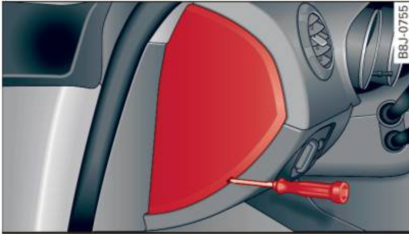
Fig. 164 End face of instrument panel: removing cover plate to access fuses
