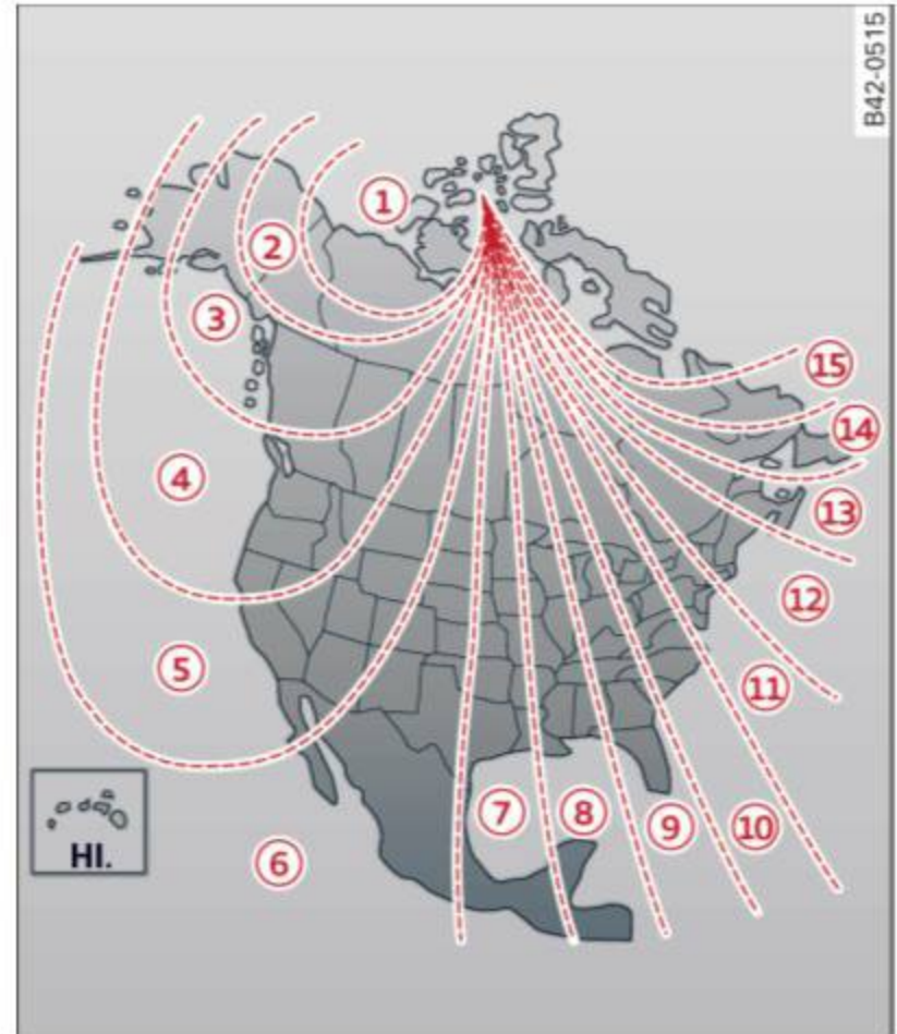
Fig. 54 North America: magnetic deflection zone boundaries
