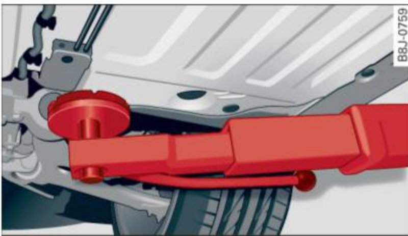
Fig. 178 Front lifting point (right side)
