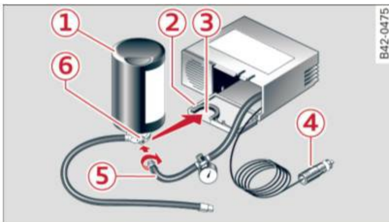
Fig. 155 Parts of the Tire Mobility System
