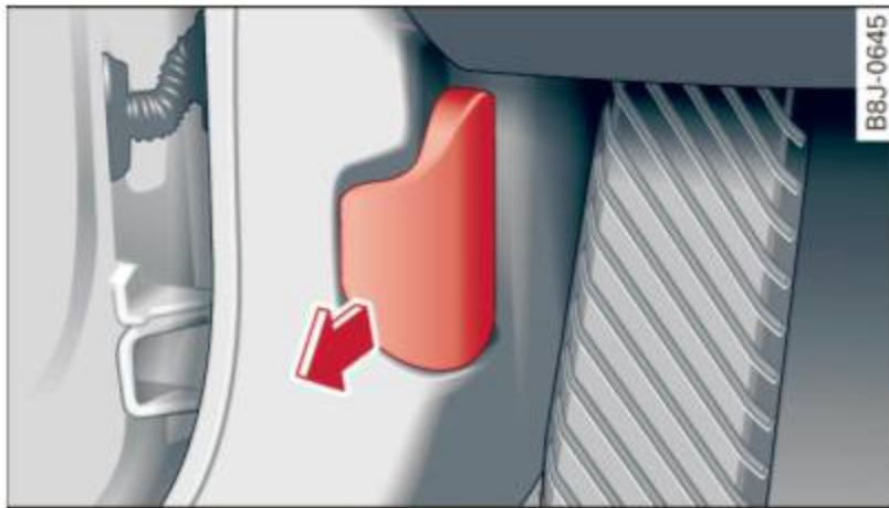
Fig. 132 Driver's side footwell: engine hood release lever
