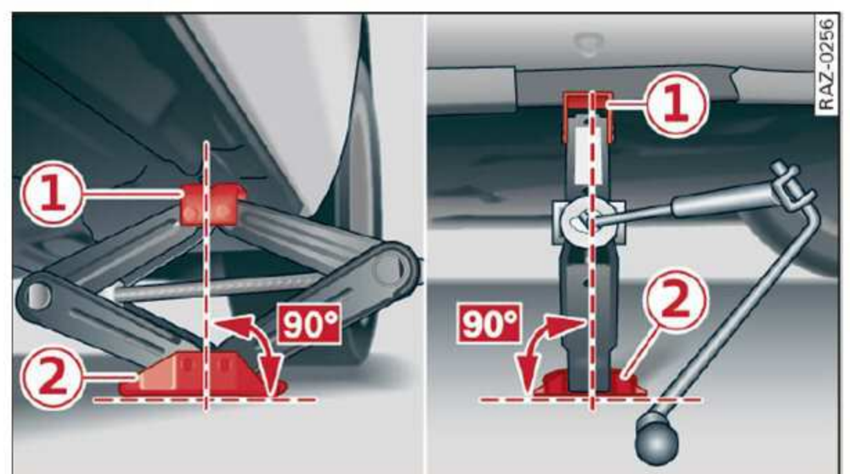
Fig. 158 Side sill: positioning the vehicle jack
