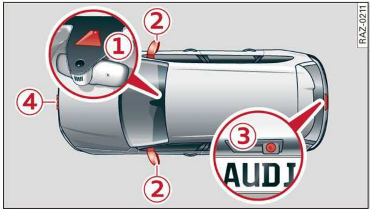
Fig. 88 Camera installation location
