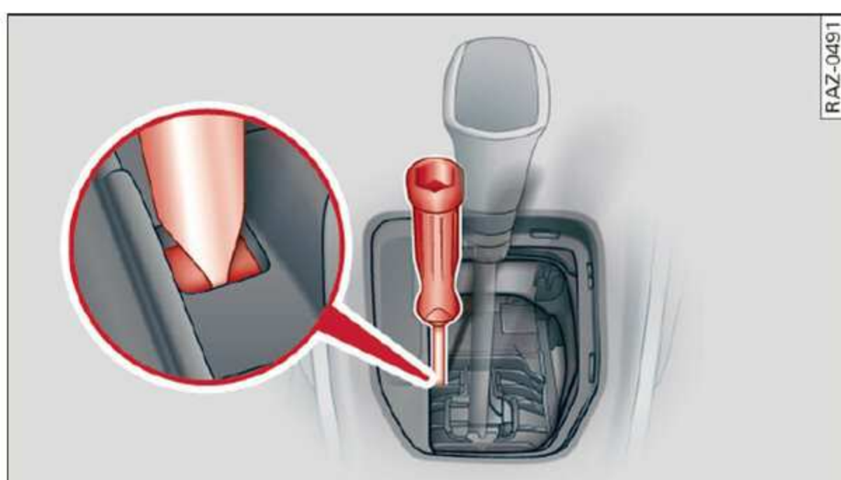
Fig. 85 Selector lever: Releasing the parking lock using the emergency release
