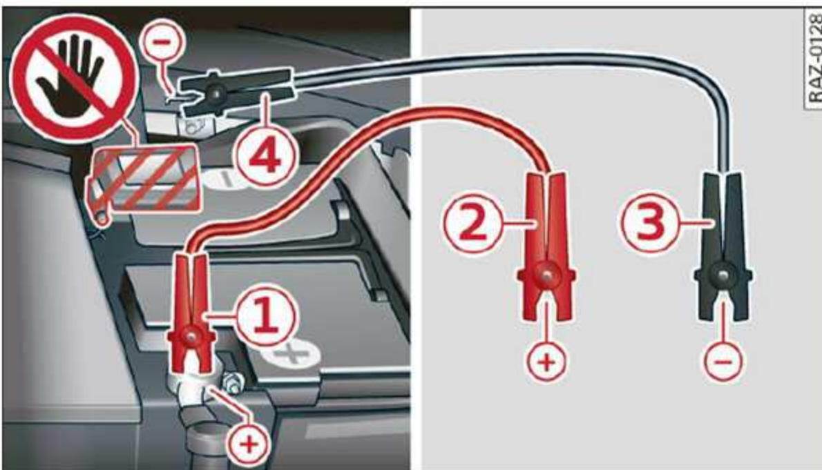
Fig. 163 Connecting the jump start cables
