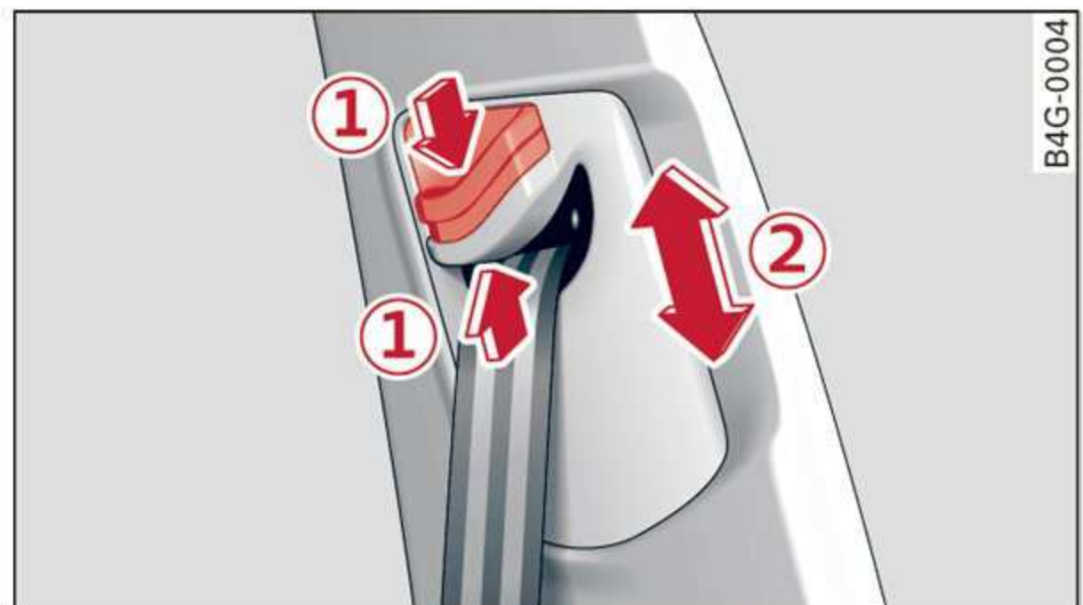
Fig. 62 Belt height adjustment for the front seats - safety belt relay
