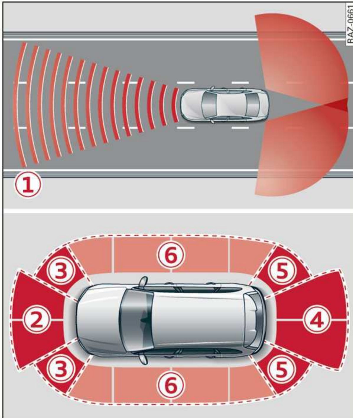
Fig. 86 Diagram: Sensor coverage area
