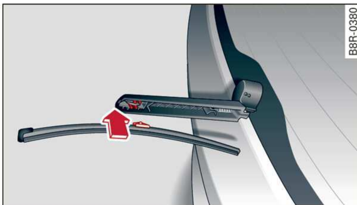
Fig. 47 Rear window wiper: removing the wiper blade
