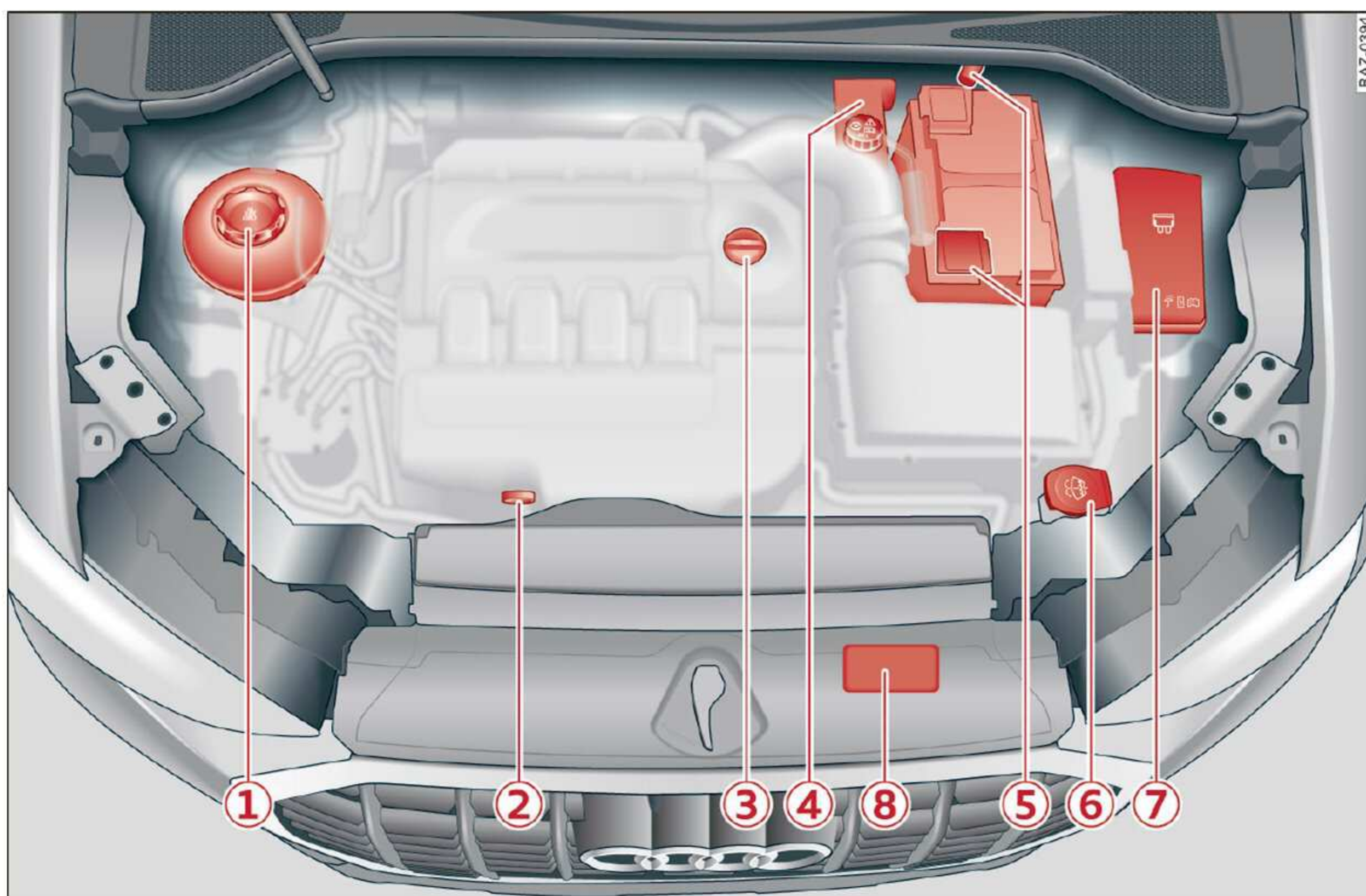
Fig. 142 Engine compartment overview: diagram
