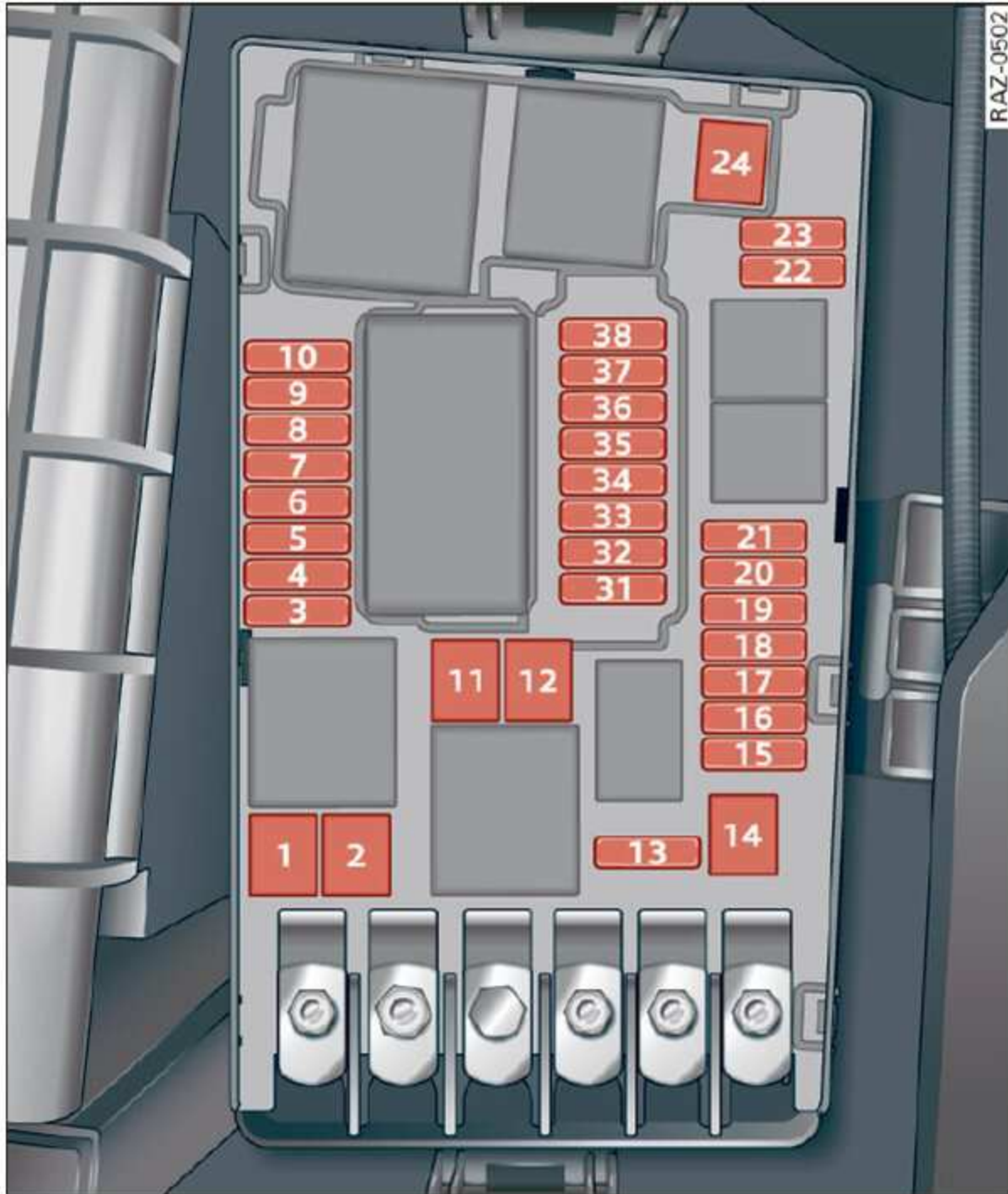
Fig. 168 Left side of engine compartment: Fuse assignment
