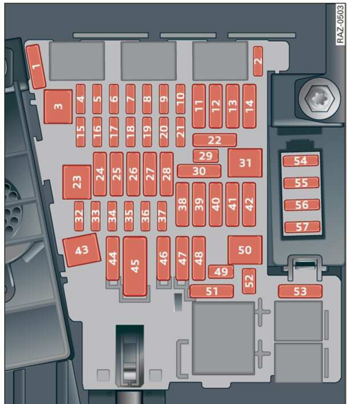
Fig. 169 Left side of cockpit: Fuse assignment
