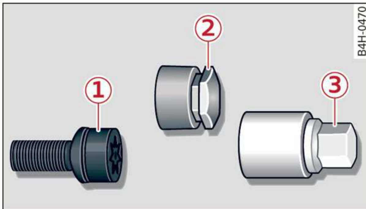
Fig. 155 Anti-theft wheel bolt with cap and adapter
