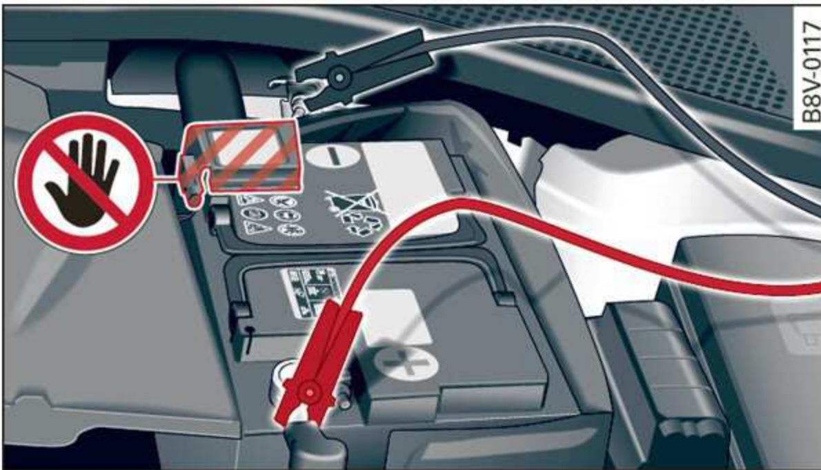
Fig. 162 Engine compartment: connectors for jump start cables or a charger
