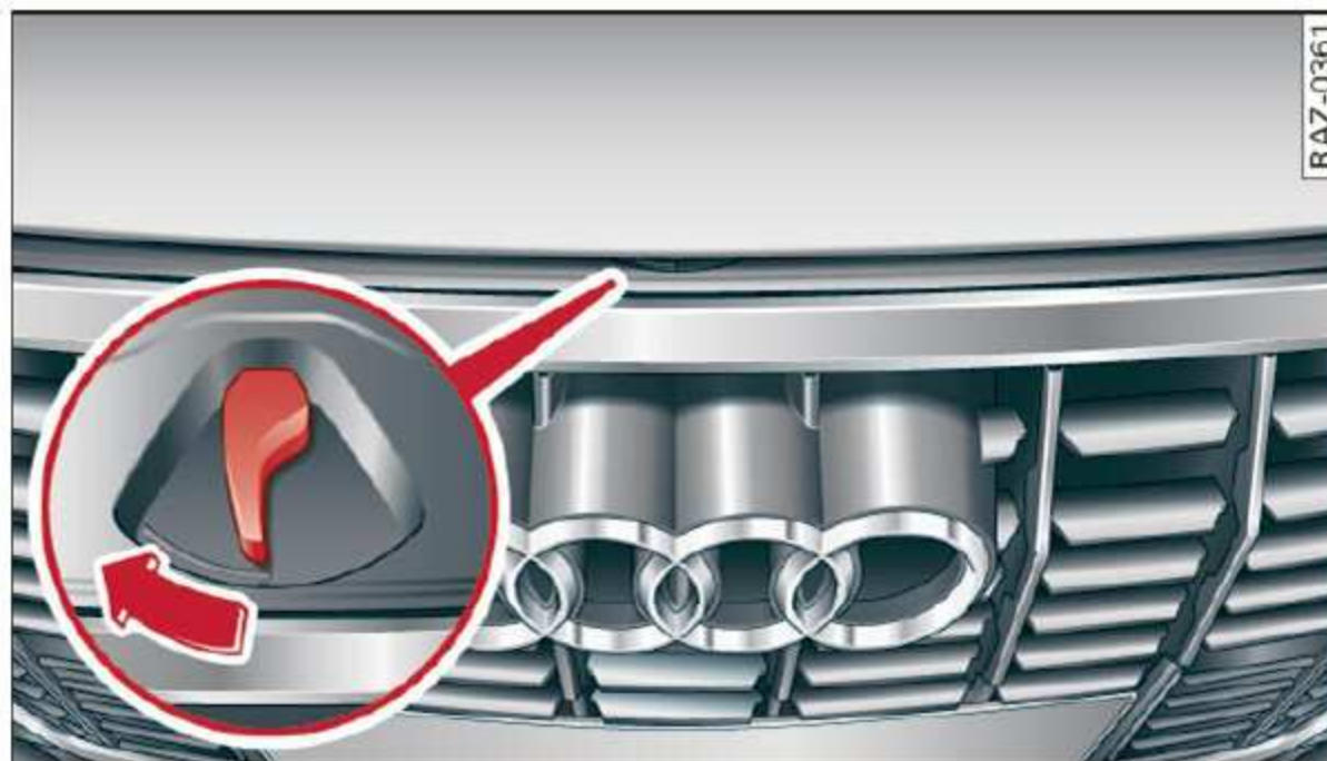
Fig. 141 Unlocked hood: lever
