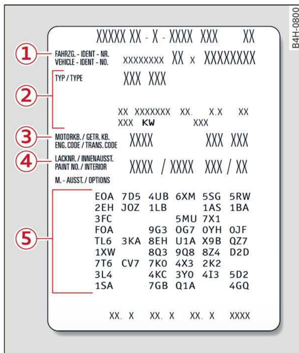
Fig. 171 Vehicle identification label
