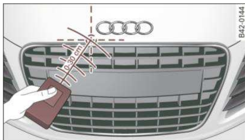
Fig. 83 Front bumper, driver side: location of transmitter unit
