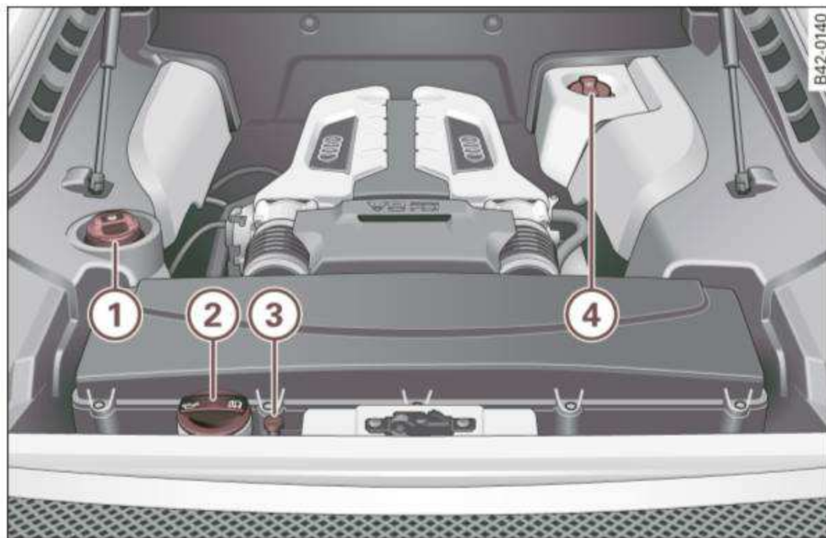
Fig. 118 Typical layout for containers, engine oil dipstick and engine oil filler cap
